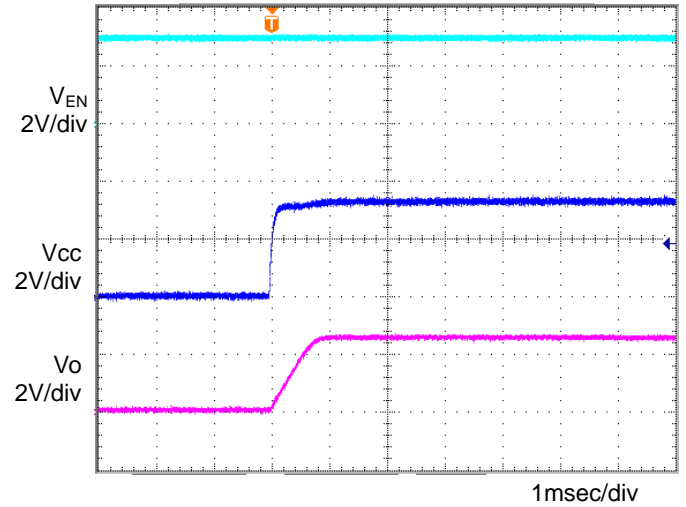
Figure 10. Input sequence 1 C_o=1\mu F, T_a=25^\circ C
