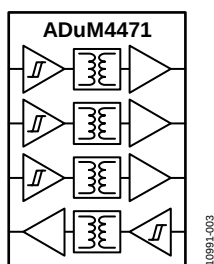
Figure 3. ADuM4471
