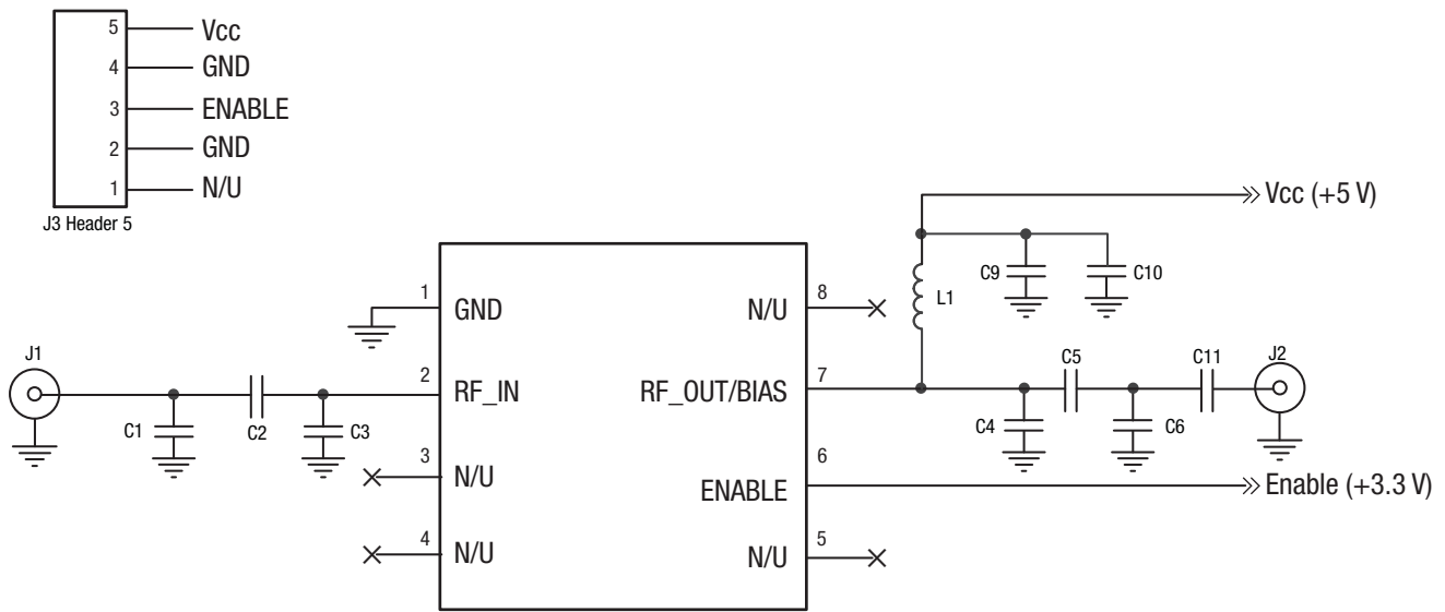
Figure 70. SKY65095-360LF Evaluation Board Schematic
