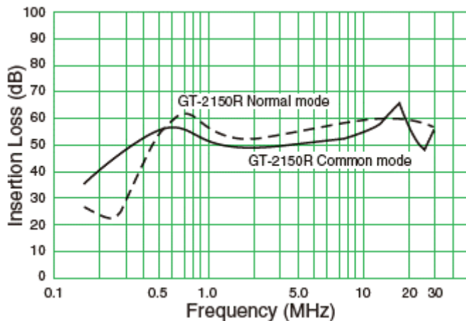
GT-2150R
