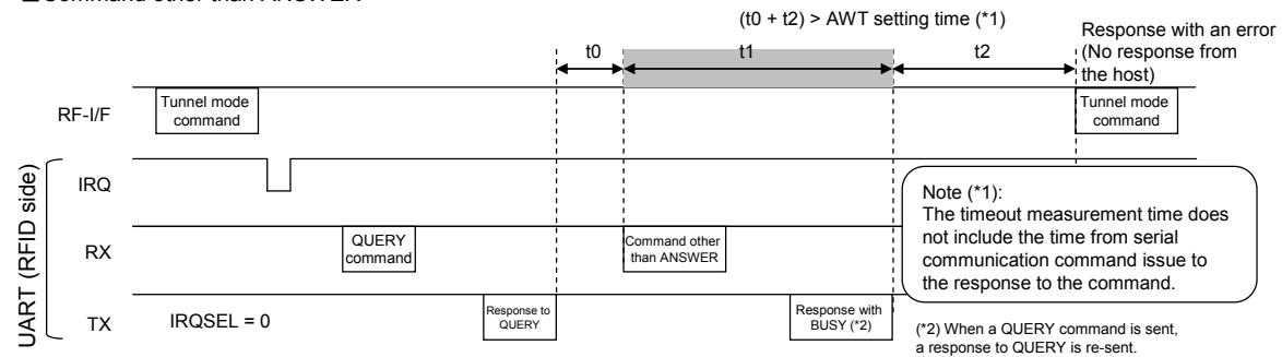
Figure 6-10 Timeout of Waiting for ANSWER Command (Command Othe than ANSWER)
