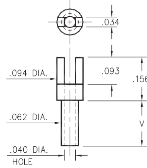
2302-X-01-XX-00-00-07-0 Swage mount in .067 hole.
