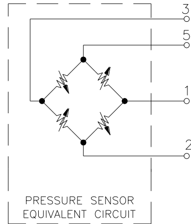
MS4425-XXXA/G
