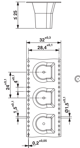
THR tape-on-reel packing
