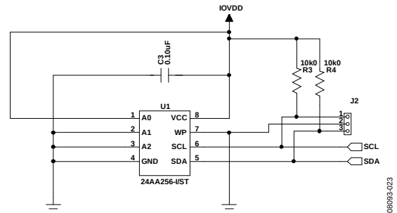
Figure 23. EEPROM Schematic
