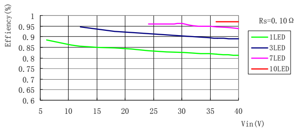
Efficiency vs. No. of LEDs L=47\mu\text{H} , R_s=0.10\text{Ohm}
