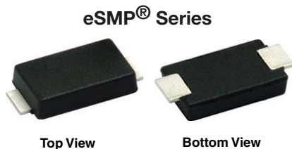
SlimSMA (DO-221AC)
