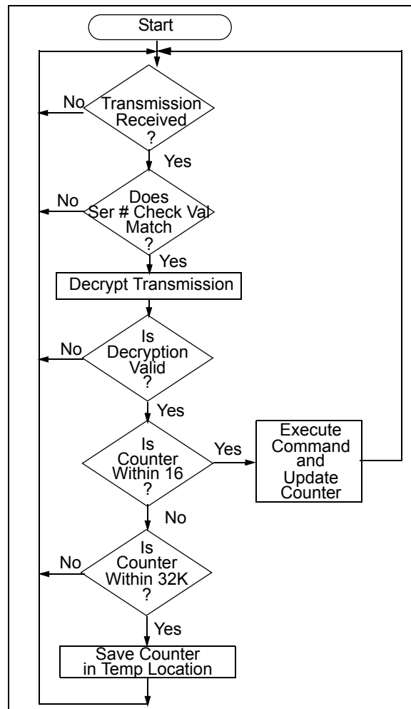
FIGURE 4-2: DECODER OPERATION
