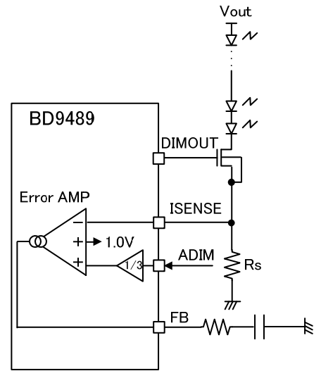
Figure 28. LED current setting example
