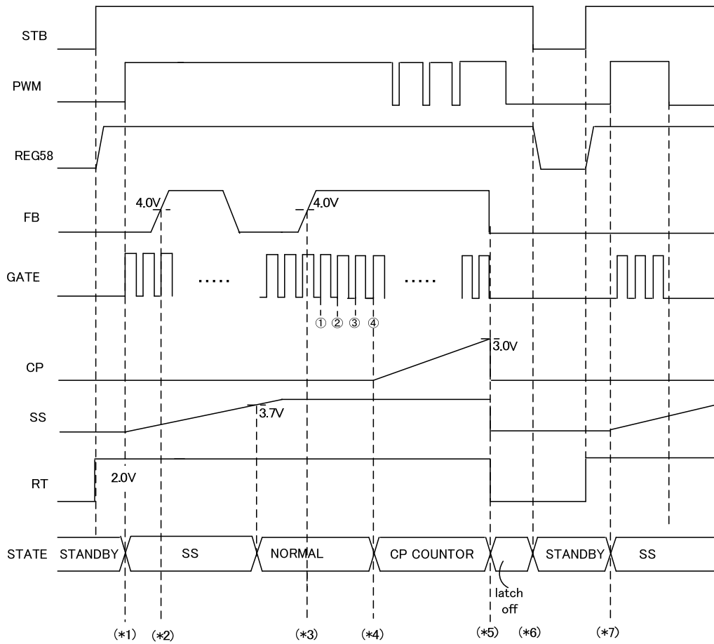
Figure 41. FBMAX Detection
