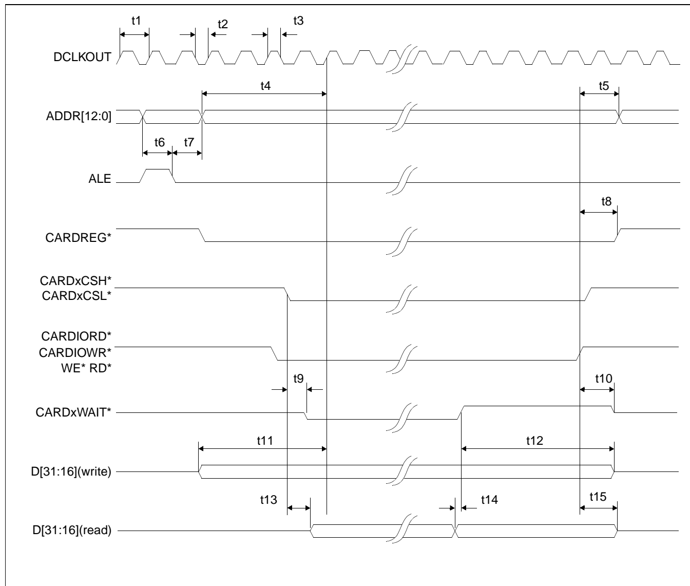
Figure 7-10: Toshiba Timing
