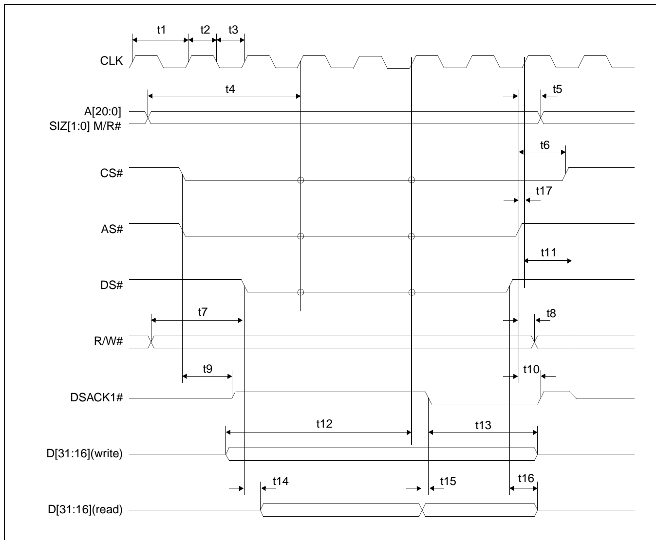
Figure 7-4: MC68030 Timing
