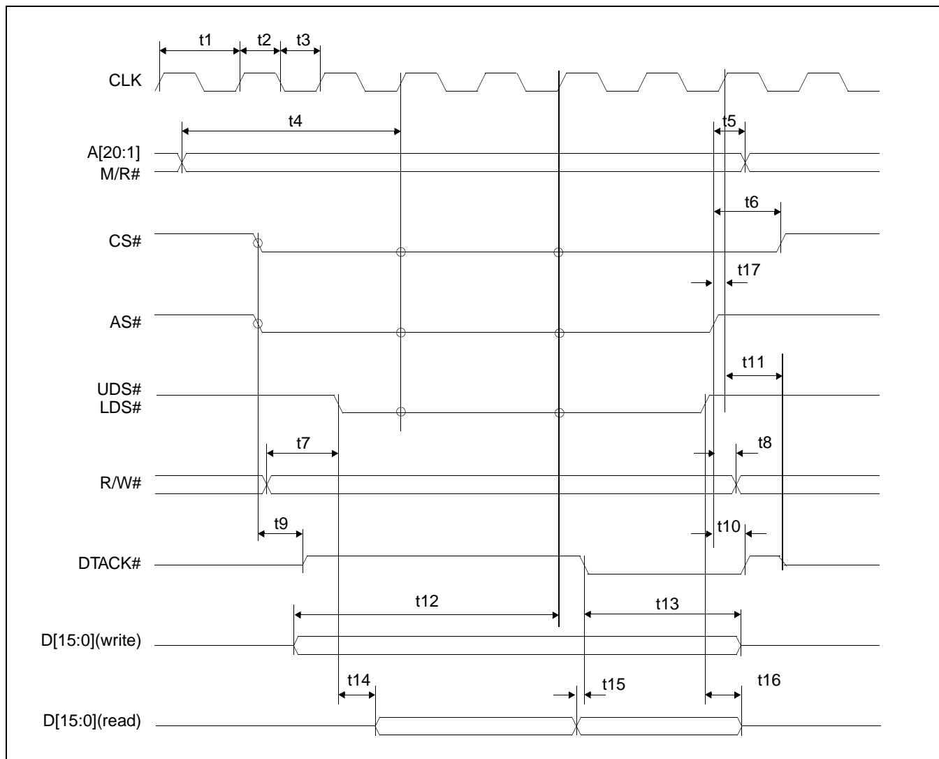
Figure 7-3: MC68000 Timing
