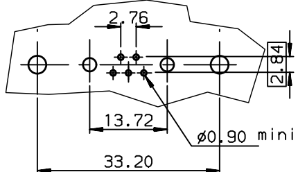
LAYOUT DIMENSIONS (after plating) CONNECTOR SIDE VIEW
