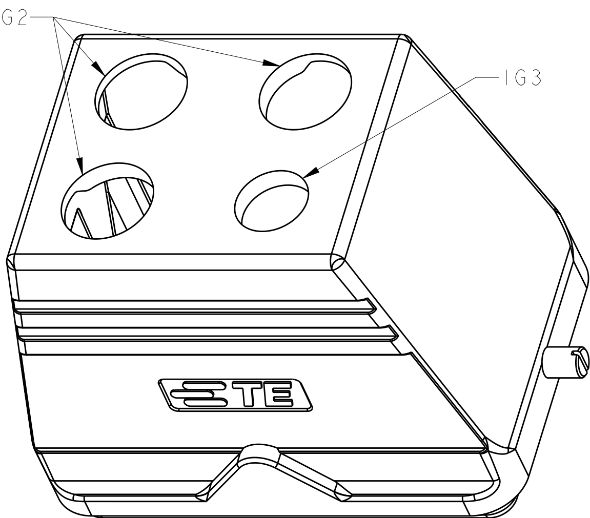
TYPE 6: TOP ENTRY( 4 HOLE) OTHER SPEC REFER TO TYPE 1
