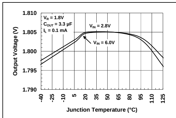
FIGURE 2-3: Output Voltage vs. Junction Temperature.
