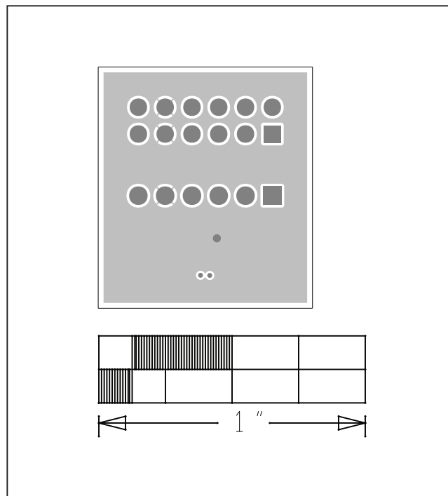
MAX31875 EV Kit—Layer 2
