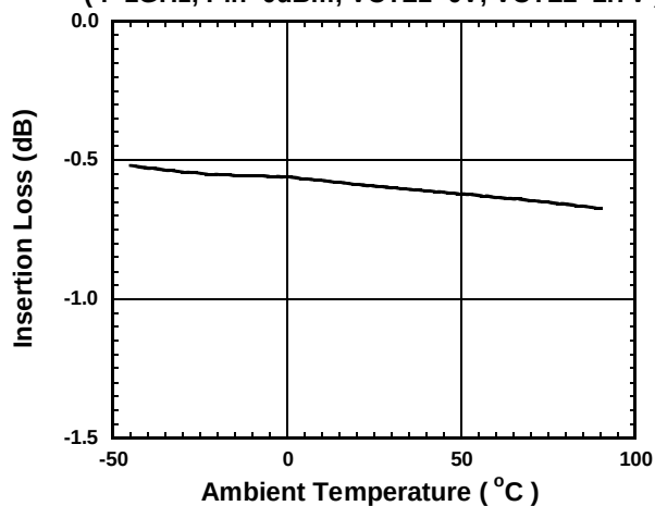
PC-P1 Loss vs. Ambient Temperature ( f=1\text{GHz} , \text{Pin}=0\text{dBm} , \text{VCTL1}=0\text{V} , \text{VCTL2}=2.7\text{V} )
