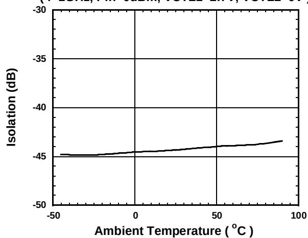
PC-P1 Isolation vs. Ambient Temperature ( f=1\text{GHz} , \text{Pin}=0\text{dBm} , \text{VCTL1}=2.7\text{V} , \text{VCTL2}=0\text{V} )
