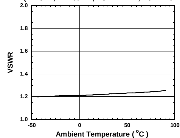
P2 VSWR vs. Ambient Temperature ( f=1\text{GHz} , \text{Pin}=0\text{dBm} , \text{VCTL1}=2.7\text{V} , \text{VCTL2}=0\text{V} )
