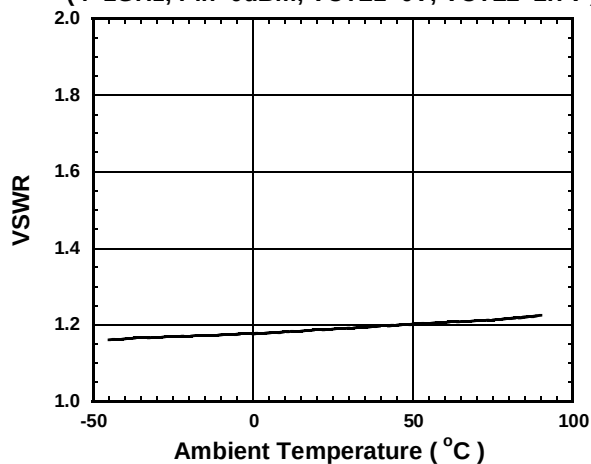
P1 VSWR vs. Ambient Temperature ( f=1\text{GHz} , \text{Pin}=0\text{dBm} , \text{VCTL1}=0\text{V} , \text{VCTL2}=2.7\text{V} )
