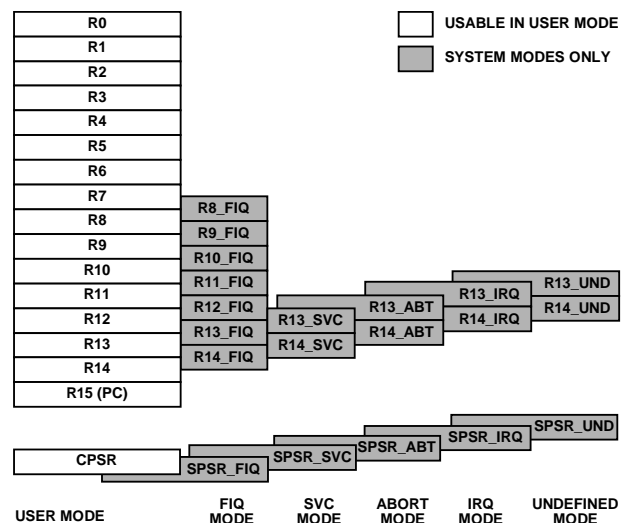
Figure 34. Register Organization
