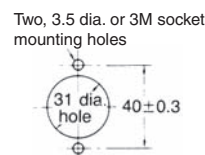
Mounting Holes
