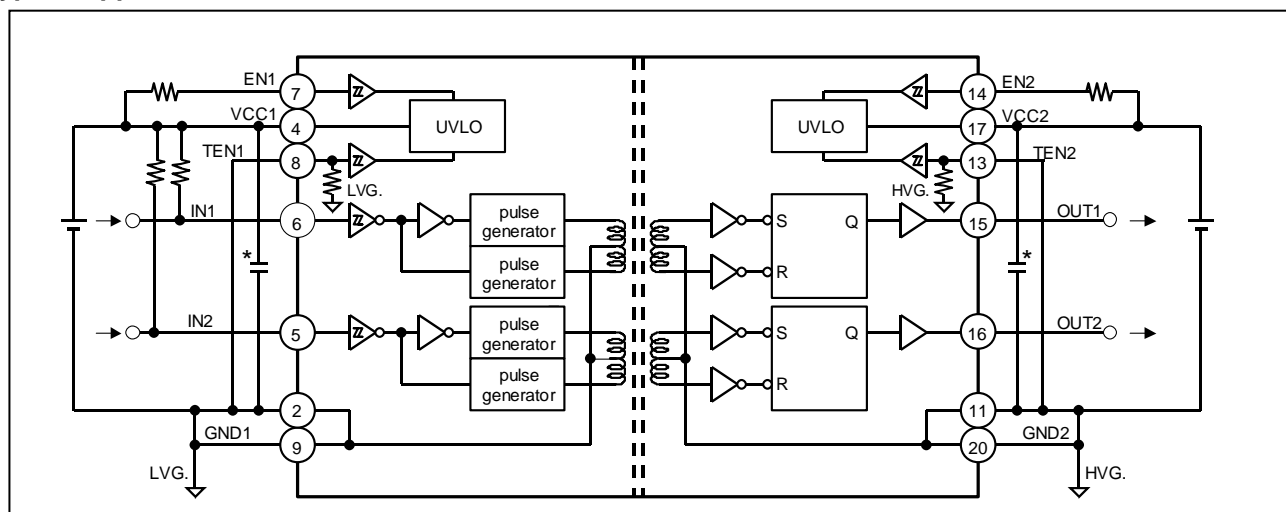
Figure 1. BM67220FV-C Application Example
