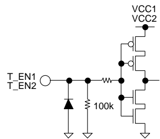
Figure 36. T_EN1, T_EN2
