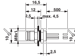
M8 flush-type plug
