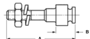
Part No. 747242-1
