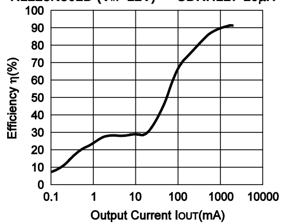
R1225N502D ( V_{IN}=12V ) CDRH127-10 \mu H
