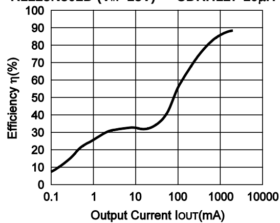
R1225N502D ( V_{IN}=15V ) CDRH127-10 \mu H
