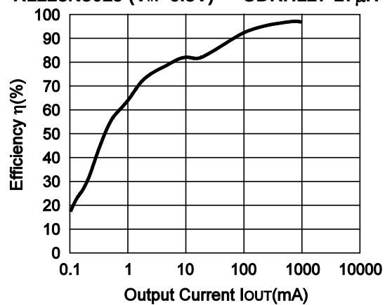
R1225N502J ( V_{IN}=6.5V ) CDRH127-27 \mu H
