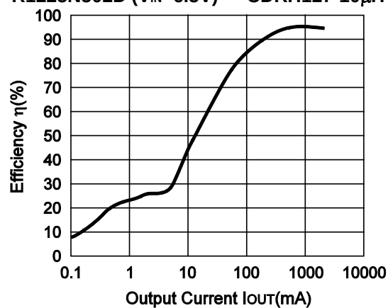
R1225N502D ( V_{IN}=6.5V ) CDRH127-10 \mu H
