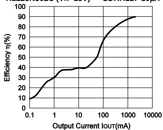
R1225N502C ( V_{IN}=15V ) CDRH127-10 \mu H
