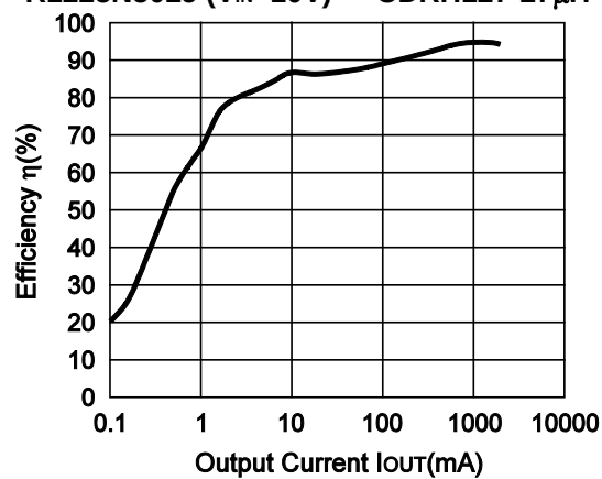
R1225N502J ( V_{IN}=10V ) CDRH127-27 \mu H
