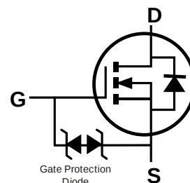
Internal Schematic
