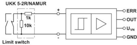
Limit switch
