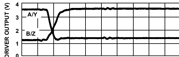
FIGURE 23. DRIVER AND RECEIVER WAVEFORMS, HIGH TO LOW (ISL83086E, ISL83088E)
