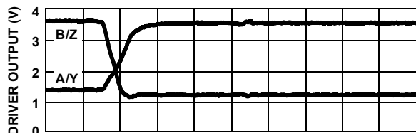
FIGURE 22. DRIVER AND RECEIVER WAVEFORMS, LOW TO HIGH (ISL83086E, ISL83088E)
