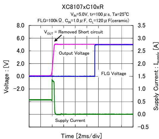
(34) Short-Circuit Transient Response
