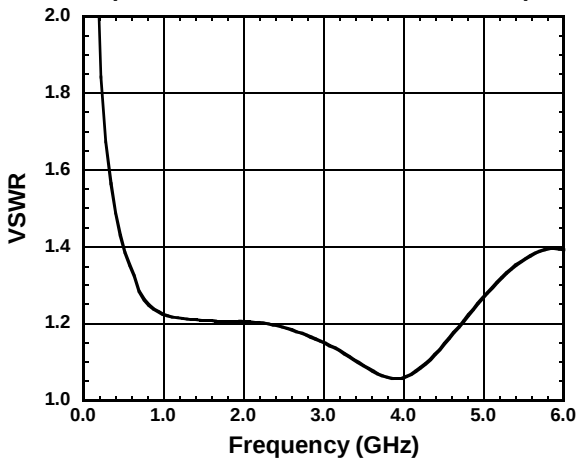
PC VSWR vs. Frequency
