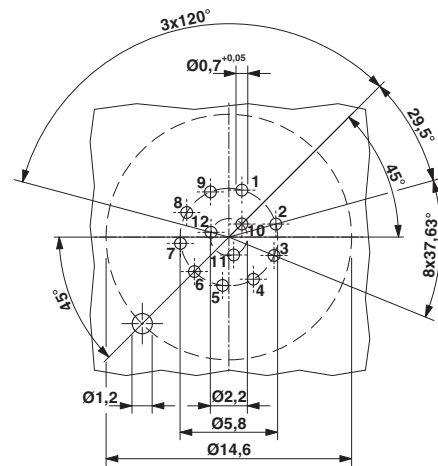
Drilling diagram
