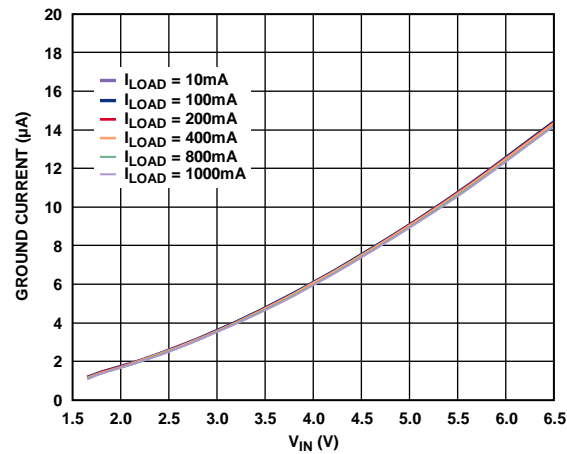
Figure 16. Ground Current vs. Input Voltage ( V_{IN} )
