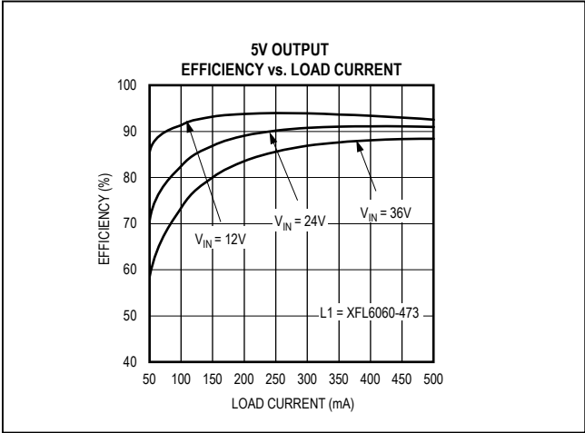
Figure 3. MAX17541G 5V Output Efficiency
