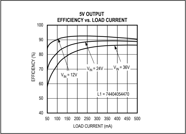
Figure 2. MAX17541G 5V Output Efficiency
