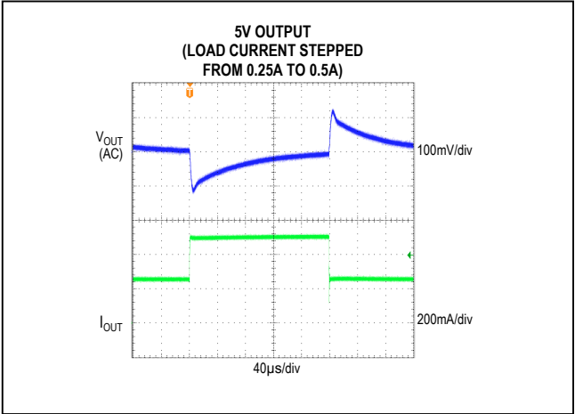
Figure 4. MAX17541G 5V Output 250mA to 500mA Load Transient
