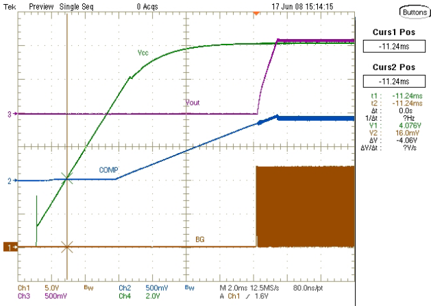
Figure 18. Start-up Sequence
