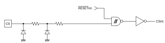
Input circuit
