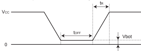
Fig. 62 Rise waveform diagram
