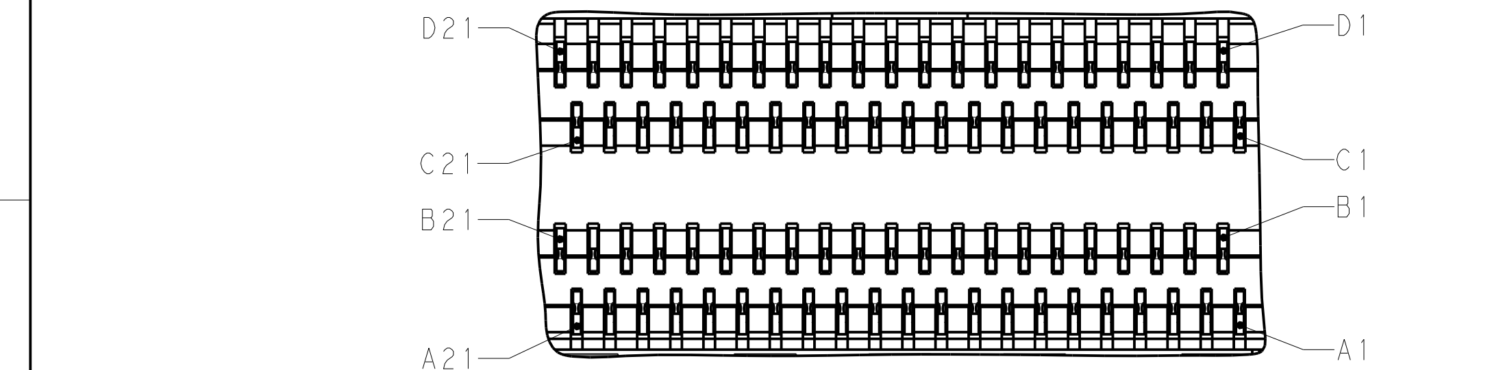
DETAIL A RECOMMENDED PIN CALLOUT SCALE 8:1
