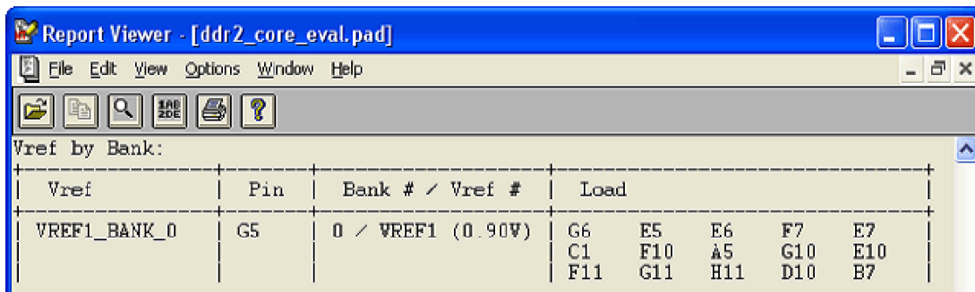
Figure 5-2. Example of VREF1 Connection Report in ispLEVER (DDR2)
