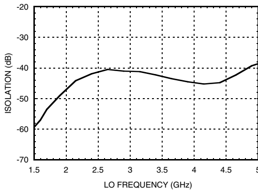
Dual Channel: LO1 to LO2 Isolation
