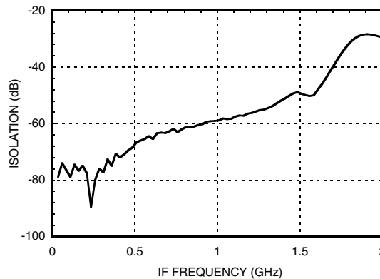
Dual Channel: IF1 to IF2 Isolation
