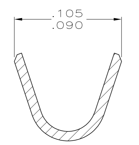
SECTION X-X INSULATION BARREL SCALE 20:1
