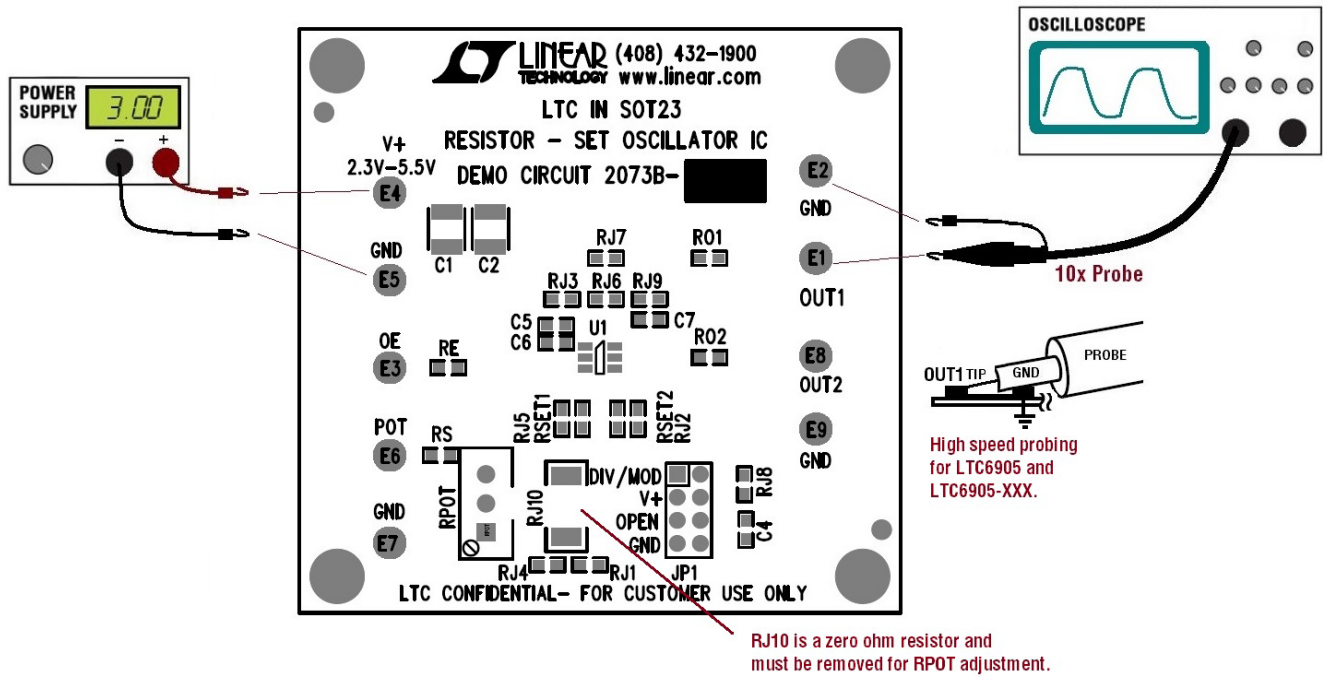
Figure 1. Test Setup
