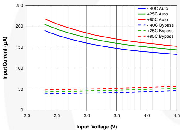
Figure 13. Quiescent Current vs. Input Voltage, Temperature and Mode, V_{OUT}=5.0\text{ V} , Forced Bypass, OCP Active
