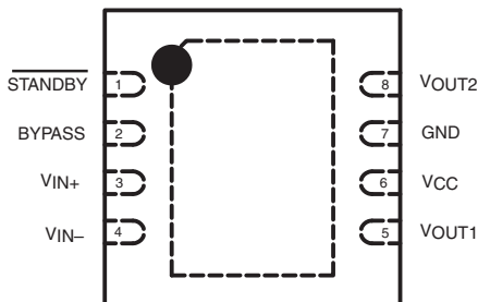
TS4990IQT - DFN8
