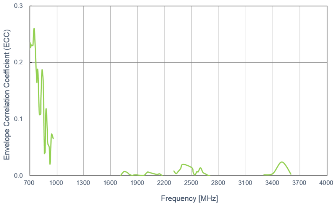
Setup in free space with 3 meter cable length
