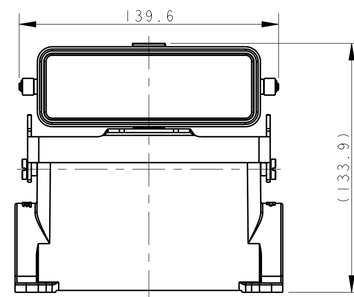
TYPE 6: HIGH BODY + SINGLE STEEL LOCKING + METAL PROTECTION COVER OTHER SPEC REFER TO TYPE 4
