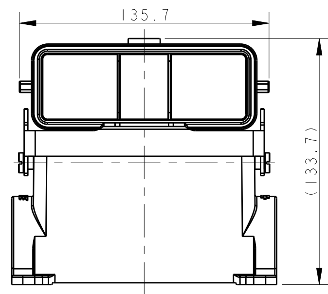
TYPE 5: HIGH BODY + SINGLE STEEL LOCKING + PLASTIC PROTECTION COVER OTHER SPEC REFER TO TYPE 4
