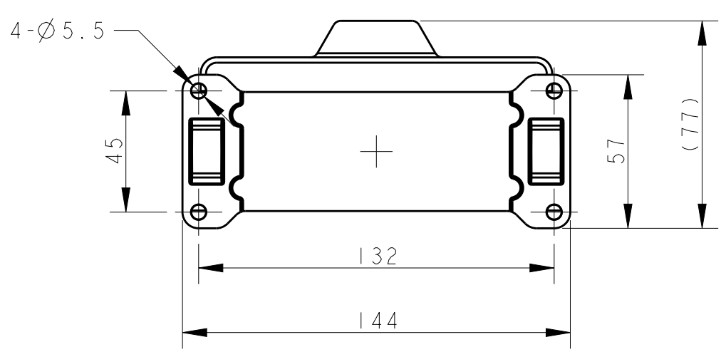
TYPE 4: HIGH BODY + SINGLE STEEL LOCKING
