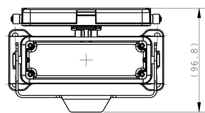
TYPE 5: HIGH BODY + SINGLE STEEL LOCKING + PLASTIC PROTECTION COVER OTHER SPEC REFER TO TYPE 4
