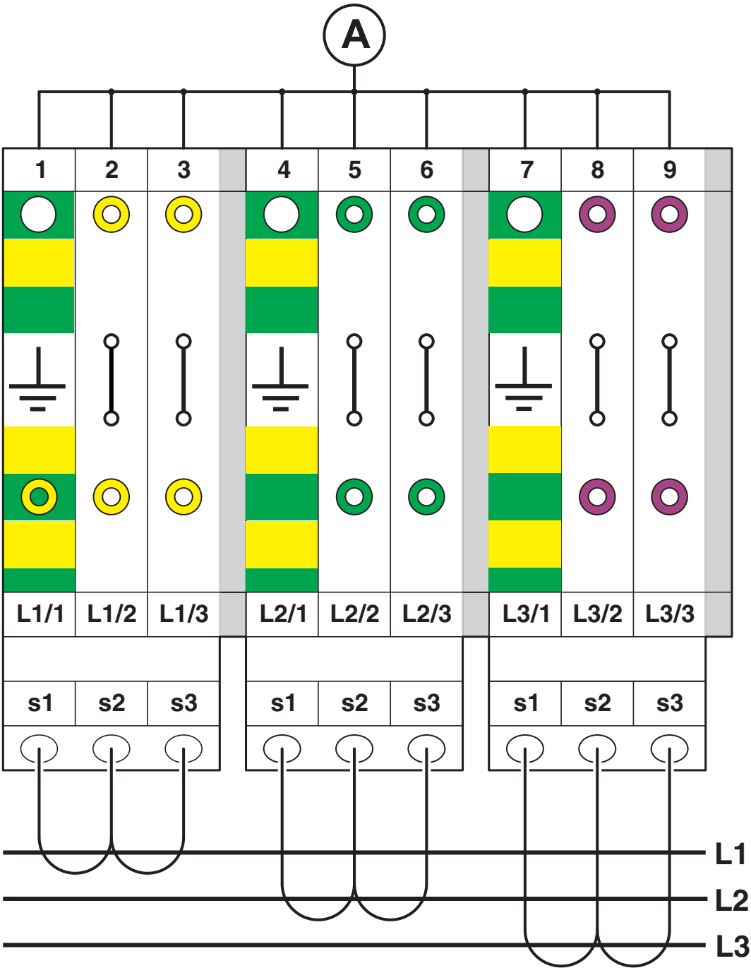
Connection diagram
