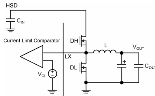
Figure 4. MIC2124 Current Limiting Circuit
