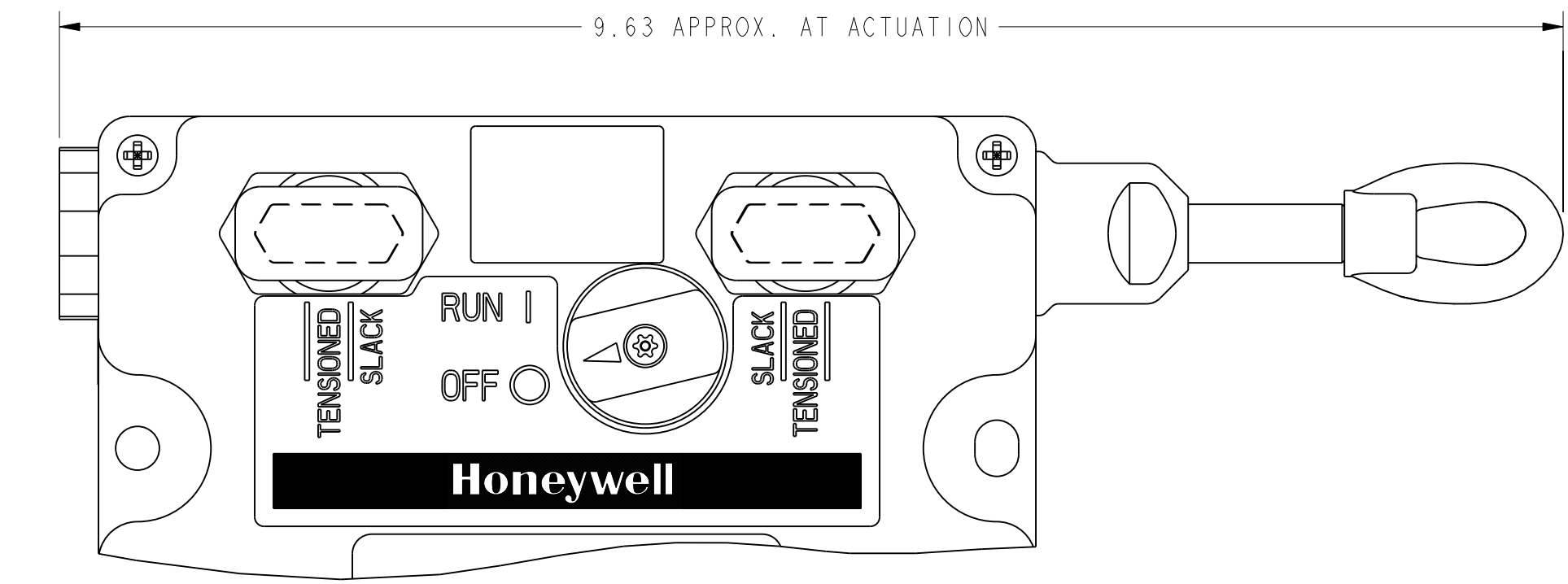
ACTUATION CODES "2" AND "3" DETAIL (ACTUATION CODE "3" SHOWN)
