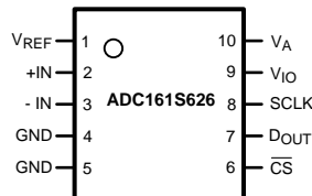
10 Pins VSSOP Package Top View
