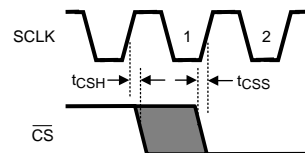
Figure 5. Valid CS Assertion Times
