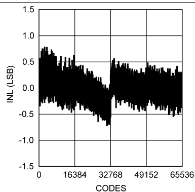
Figure 8. INL - 250 kSPS
