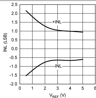
Figure 12. INL vs. V_{REF}
