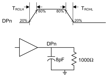
FIGURE 15. LVCMOS Output Load and Transition Times
